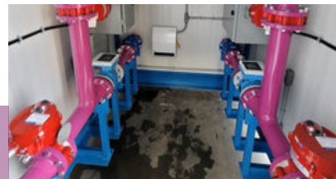
Above: Station with small booster pump to increase pressure at the station and reduce burden on the WWTP. Below: Custom large simultaneous dual fill station with upper and lower fill points. Stations like this can also be built to manage different reuse types and points.
