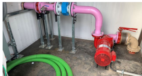
Above: Station with small booster pump to increase pressure at the station and reduce burden on the WWTP. Below: Custom large simultaneous dual fill station with upper and lower fill points. Stations like this can also be built to manage different reuse types and points.
