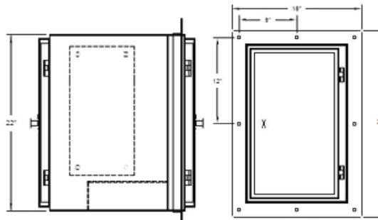
Above: Thru-Wall
